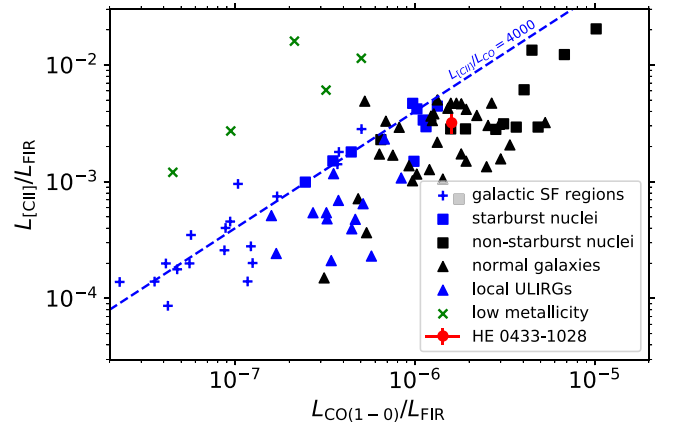
Figure 5. Position of HE 0433-1028 in the L_{\text{CO}(1-0)}/\text{FIR} - L_{[\text{C II}]} / L_{\text{FIR}} plane compared to data points for normal galaxies, ultraluminous infrared galaxies, galactic star formation regions, galactic nuclei, and low-metallicity galaxies from Stacey et al. (2010) and De Breuck et al. (2011, and references therein). A typical starburst [C II]/CO line ratio of \sim 4000 is indicated.
