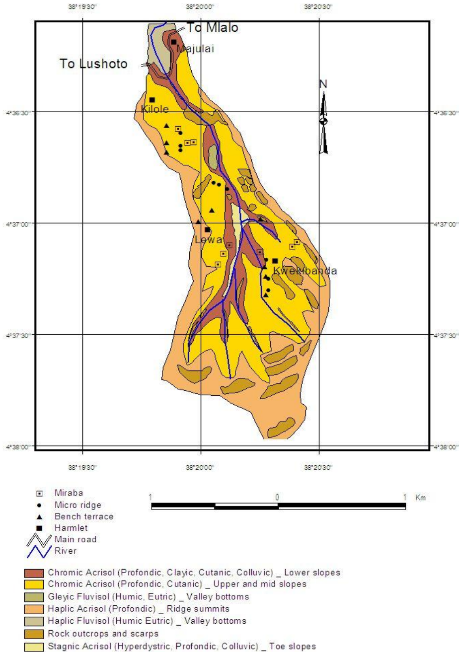
Fig. 4. Soil map of Majulai watershed, Lushoto, Tanzania
