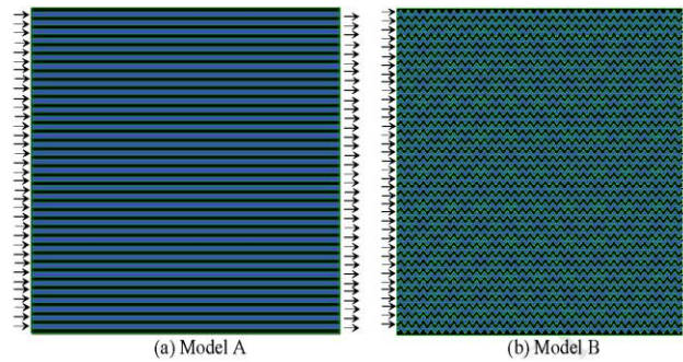
Fig. 2. Parallel and serrated flow channels
