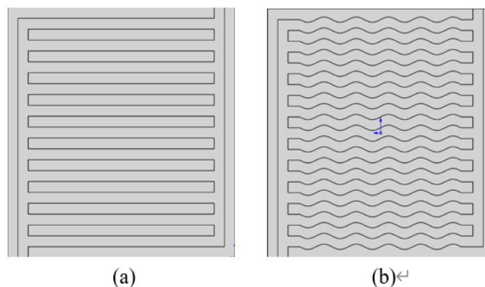
Fig. 1. Wave channel and straight channel
