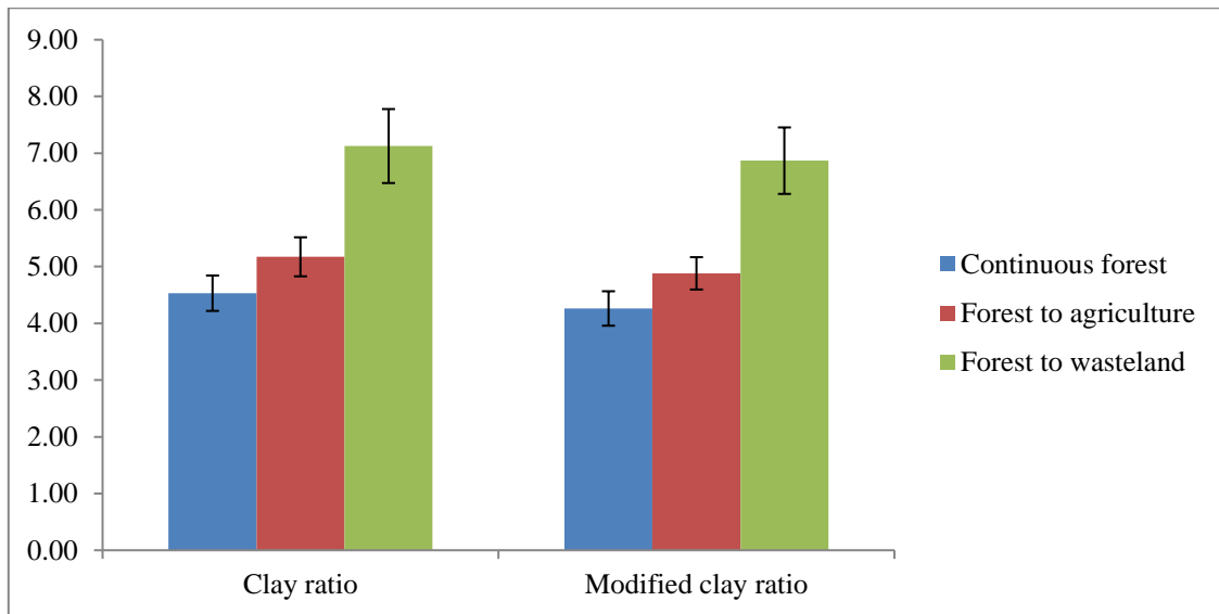
Fig. 2. Clay ratio and Modified clay ratio in continuous forest and land use conversion from forest
