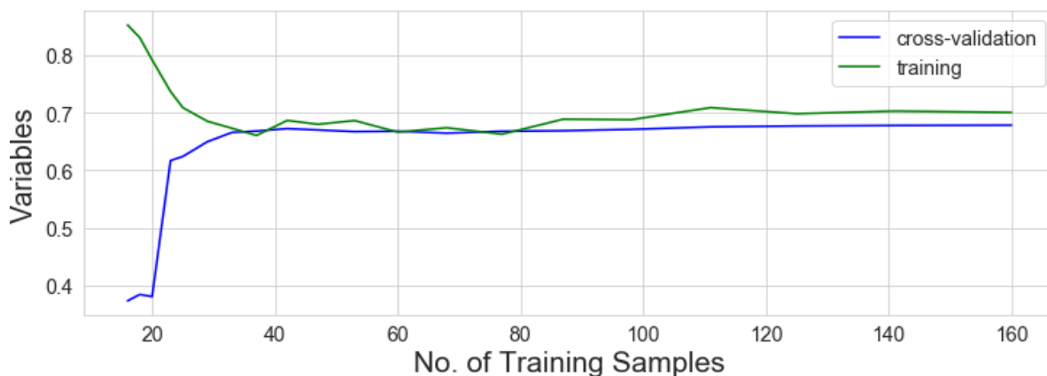
Fig. 5. The SVM learning Curve
