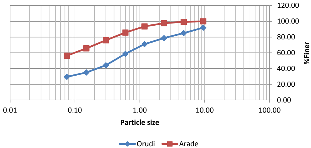
Fig. 5. Particle size distribution of Arade and Orudi samples
