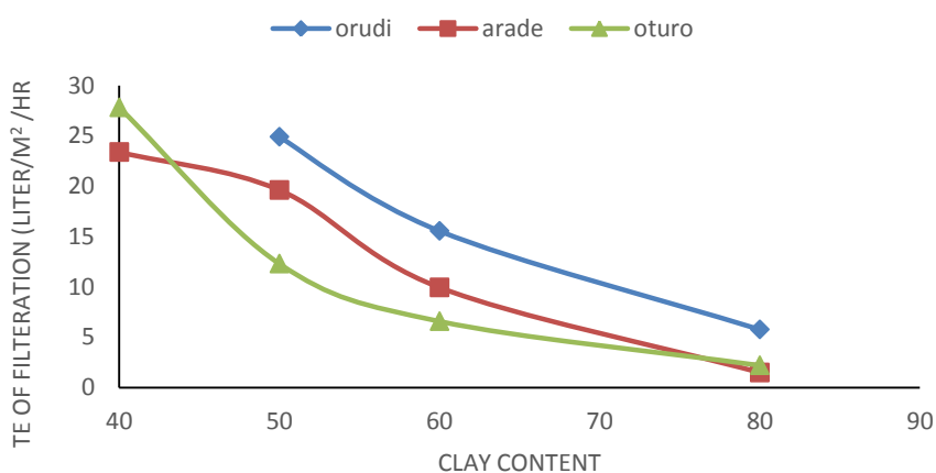
Fig. 8. Effect of % Content of Samples Clay on rate of filtration
