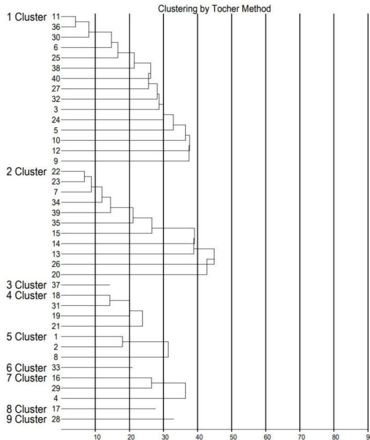
Fig. 1. Dendrogram showing the clustering pattern of 40 mung bean genotypes
