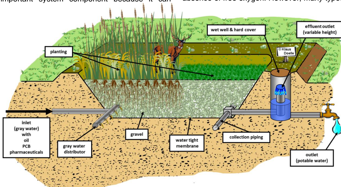
Fig. 5. Sketch of a Subterranean Flow Constructed Wetland [22]
