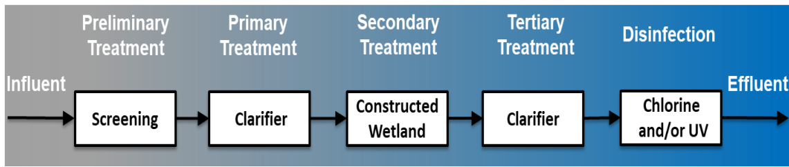
Fig. 1. Application of a Constructed Wetland Treatment Process [21]
