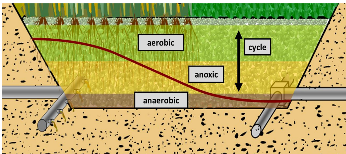
Fig. 8. Tidal Operation of a Subterranean Flow Constructed Wetland Cell [32]
