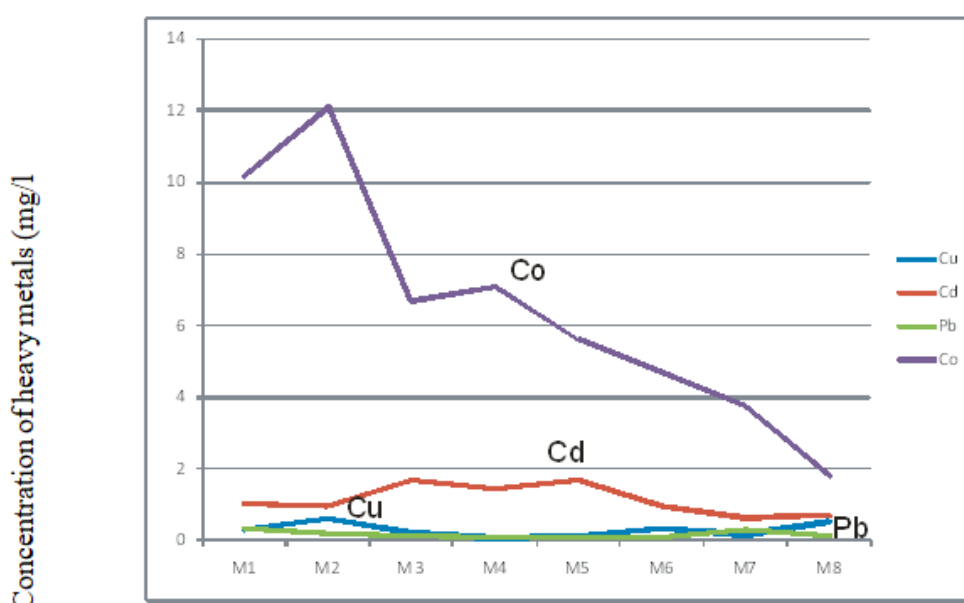
Fig. 1. Trend of accumulation of heavy metals at sampling point 1 in Wulmi River Months (May – December 2017)
