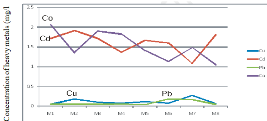
Fig. 5. Trend of accumulation of heavy metals at sampling point 5 in Wulmi River Months (May – December 2017)
