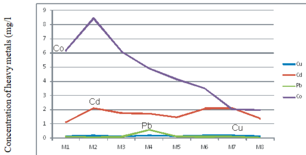
Fig. 4. Trend of accumulation of heavy metals at sampling point 4 in Wulmi River Months (May – December 2017)
