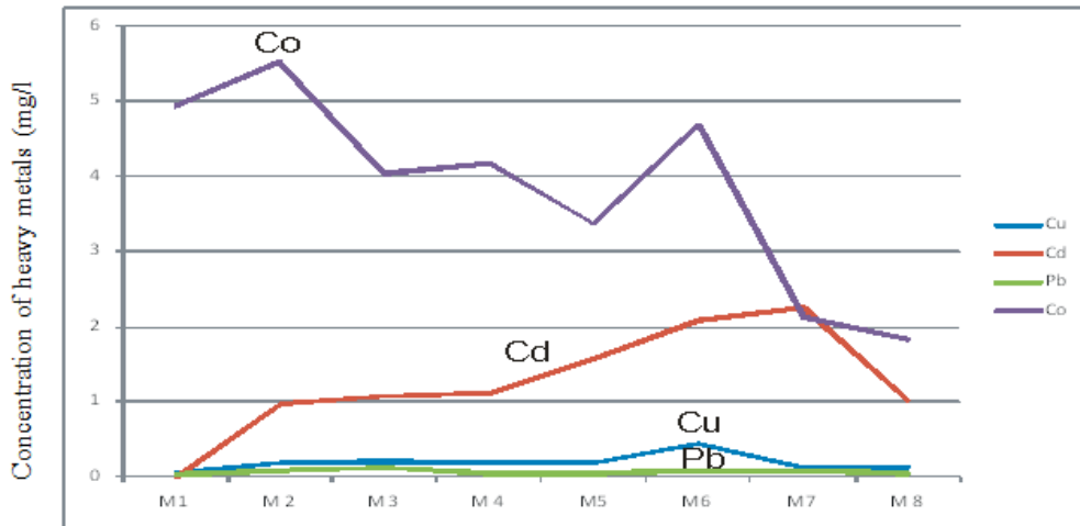
Fig. 2. Trend of accumulation of heavy metals at sampling point 2 in Wulmi River Months (May – December 2017)
