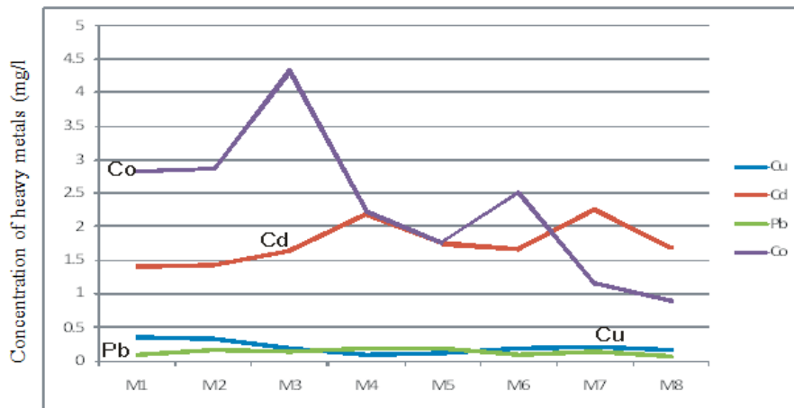
Fig. 2. Trend of accumulation of heavy metals at sampling point 2 in Wulmi River Months (May – December 2017)
